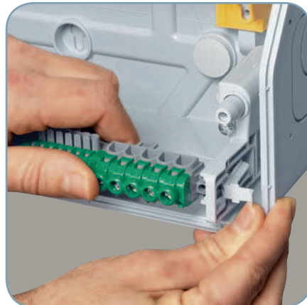
▲ Enclosures can be fitted with terminal blocks, which can easily be repositioned at the top and bottom of the box
